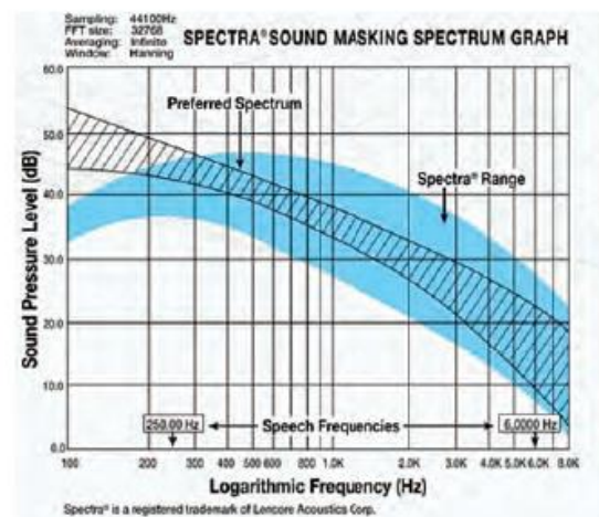
Sound Masking Spectrum Graph
